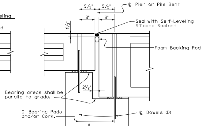
STEPPED PIER OR PILE BENT
