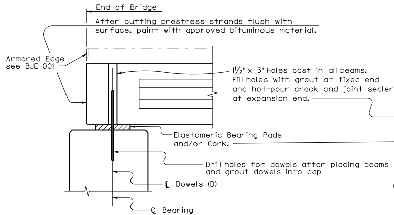
ABUTMENT OR END BENT
