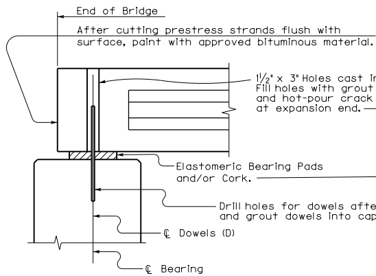
ABUTMENT OR END BENT
